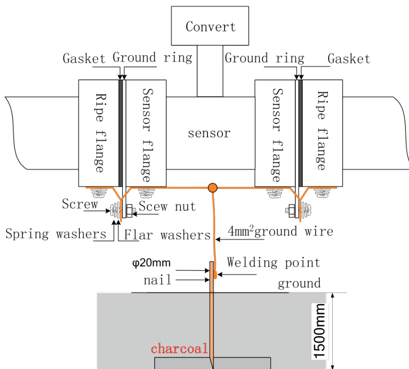
Fig.4.4(f) Grounding
